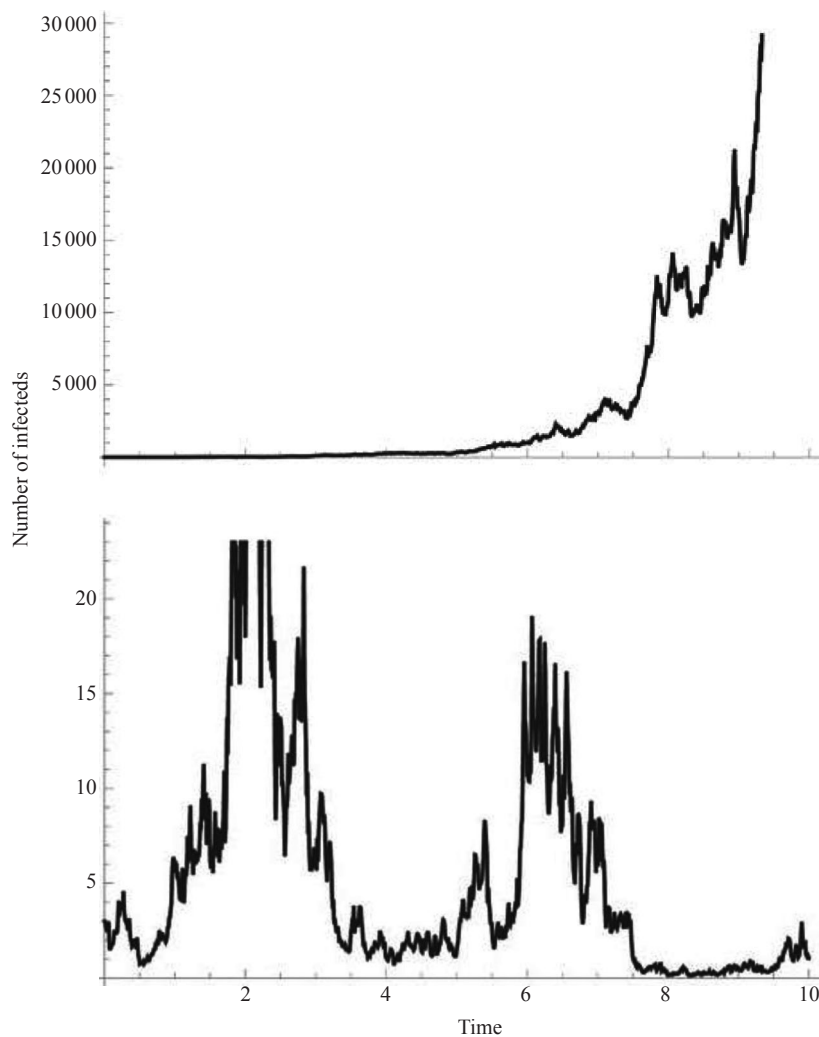
Figure 2. Simulations of equation (1) using the white noise ( H = 1/2 ) ItoProcess construct in Mathematica: \alpha = 1 , critical \sigma = (2)^{1/2} , initial number of infecteds, N_0 = 3 . The upper trace has \sigma = 0.5 , the lower has \sigma = 1.6 . One thousand time steps. While the upper outbreak eventually reaches tens of thousands, the lower remains under 100.
